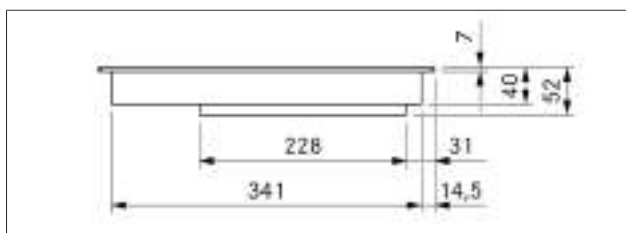
Fig. 3.9 PKFI3 appliance dimensions front view
