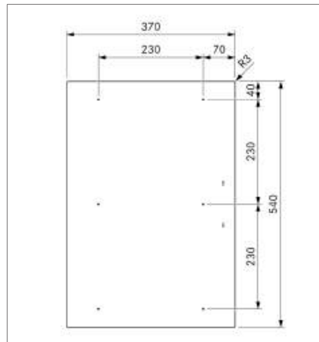
Fig. 3.8 PKF13 appliance dimensions from above
