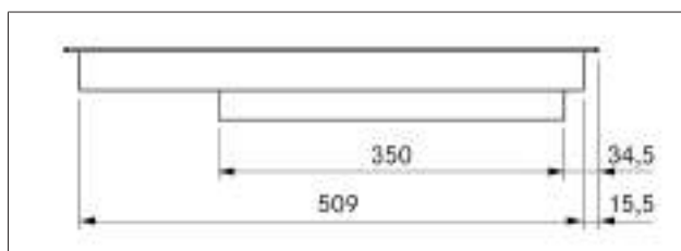
Fig. 3.19 PKC3 appliance dimensions side view
