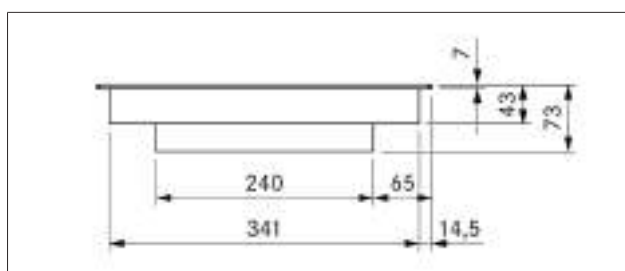
Fig. 3.18 PKC3 appliance dimensions front view
