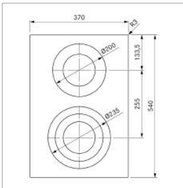
Fig. 3.17 PKC3 appliance dimensions from above
