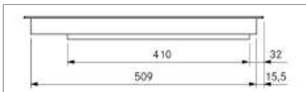
Fig. 3.10 PKFI3 appliance dimensions side view
